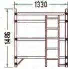
3 Rung Ladder Frame Double Width (SWL3) 双宽三级直爬梯架
