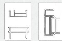
双层专利设计, 2层结构受力更稳定 Double-layer patented design, more stronger
