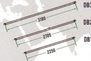
Diagonal Braces (RED) DB3/DB2/DB1 斜杆 (红色)
