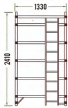
5 Rung Ladder Frame Double Width (SWL5) 双宽五级直爬梯架
