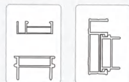
双层专利设计, 2层结构受力更稳定 Double-layer patented design, more stronger
