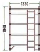
4 Rung Ladder Frame Double Width (SWL4) 双宽四级直爬梯架
